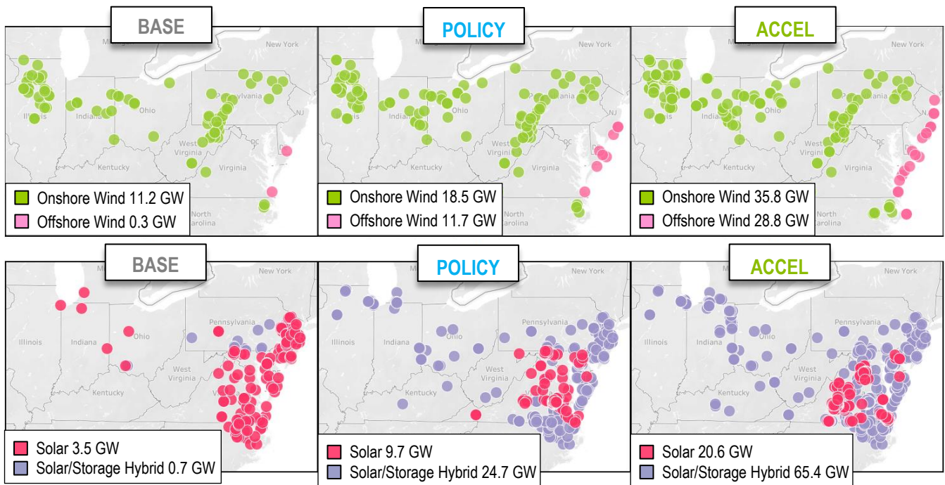
Figure 1. Renewable Generation Expansion in Policy and Accelerated Scenarios
