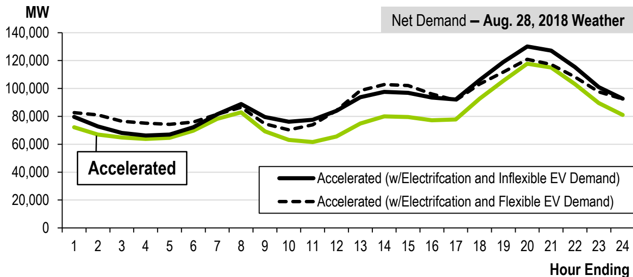
Figure 6. Summer Load Shape With Electrification
