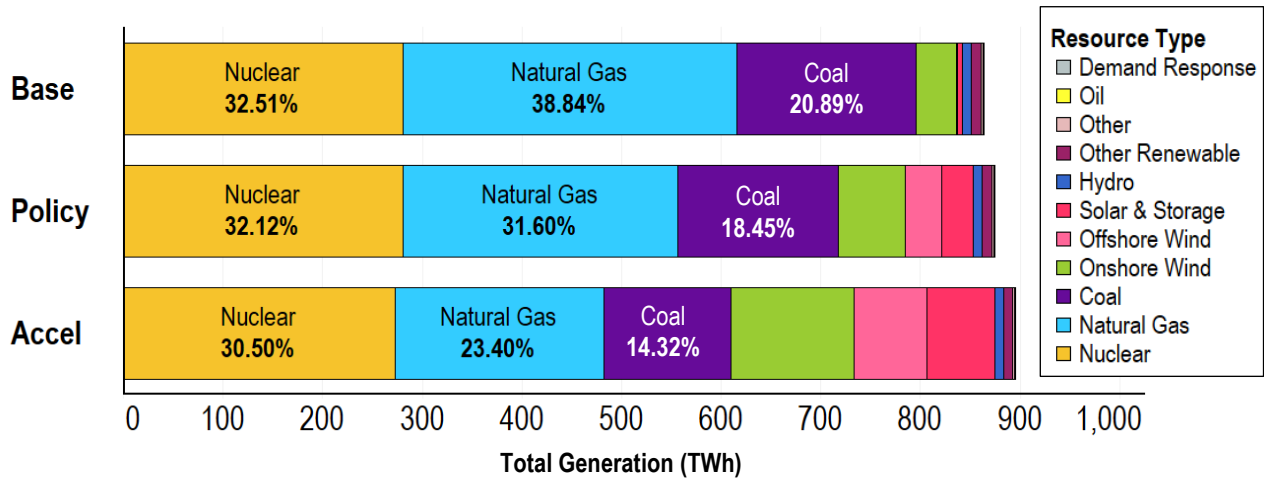
Figure 11. Annual Energy Generation by Fuel Type (TWh)
