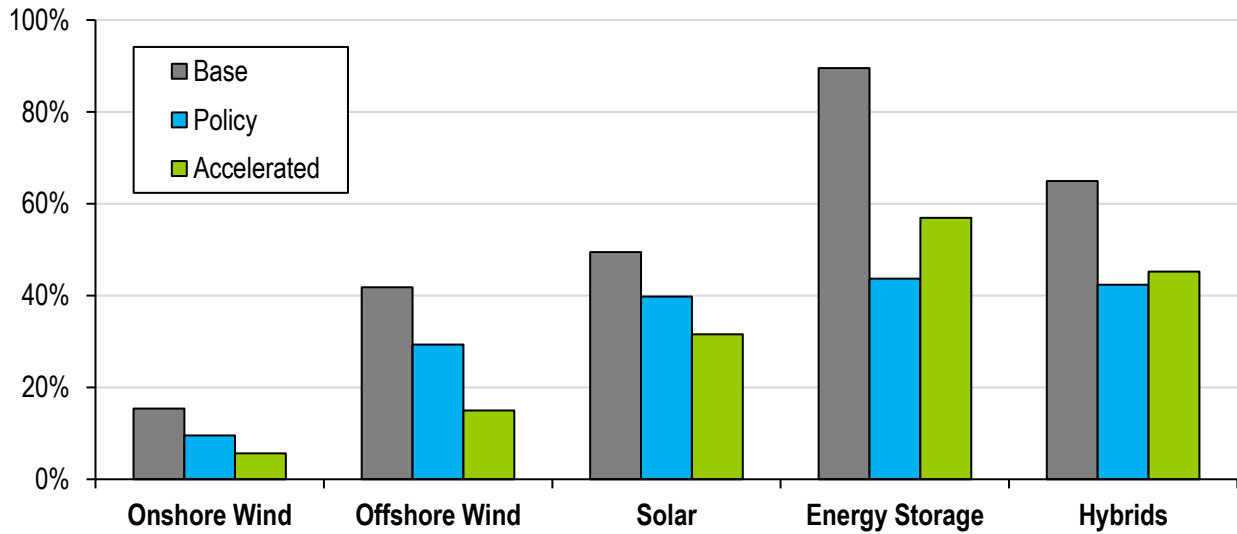
Figure 5. Effective Load Carrying Capability Results by Resource Type
