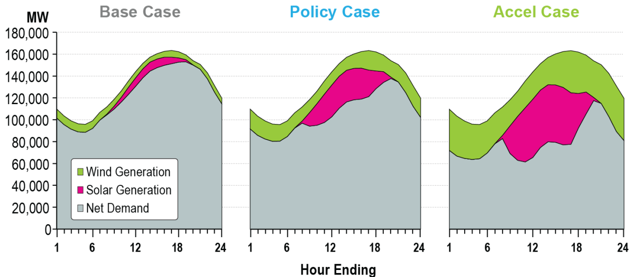
Figure 4. Aug. 28, 2018, Demand for Base, Policy and Accelerated Scenarios
