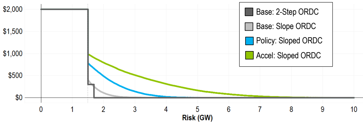
Figure 12. Two-Step and Downward-Sloping ORDC Curves
