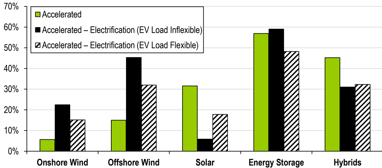
Figure 9. Effective Load Carrying Capability Results by Resource Type – With Electrification
