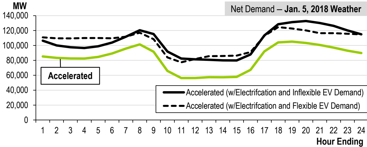
Figure 7. Winter Load Shape With Electrification
