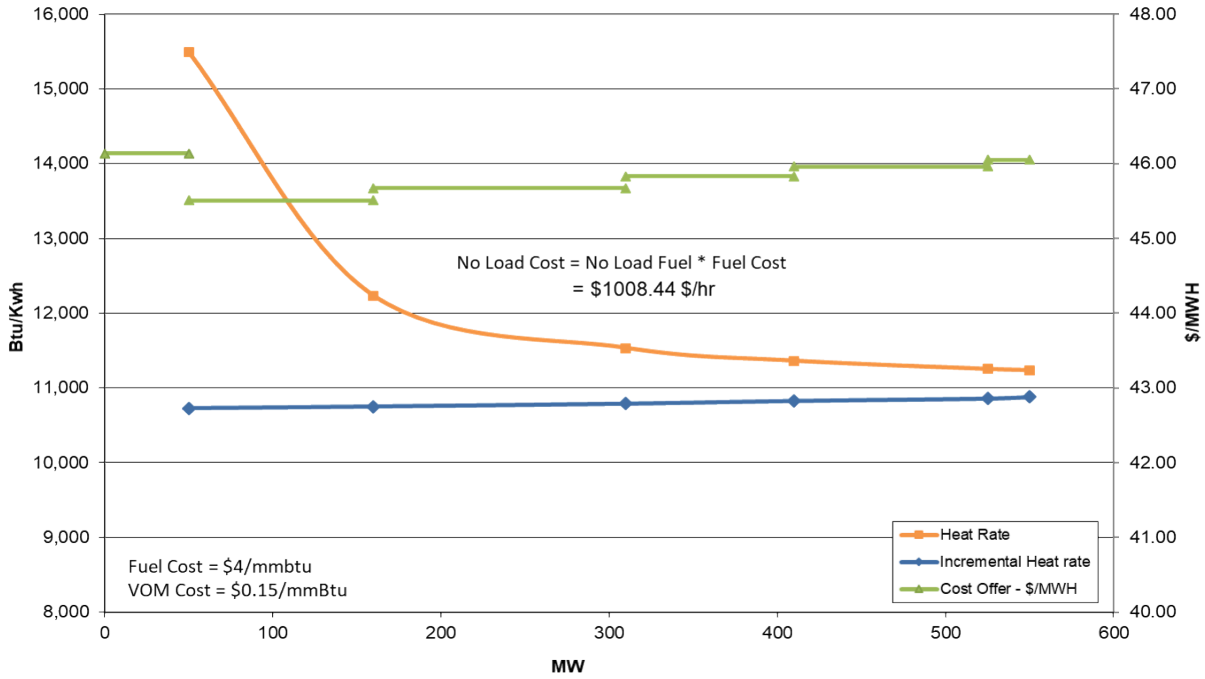
Typical Natural Gas Heat Rate & Cost Curves for 550 MW Steam Unit
