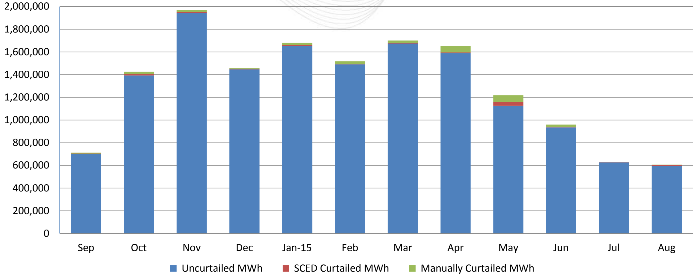
Monthly Wind Power Generation and Curtailments
