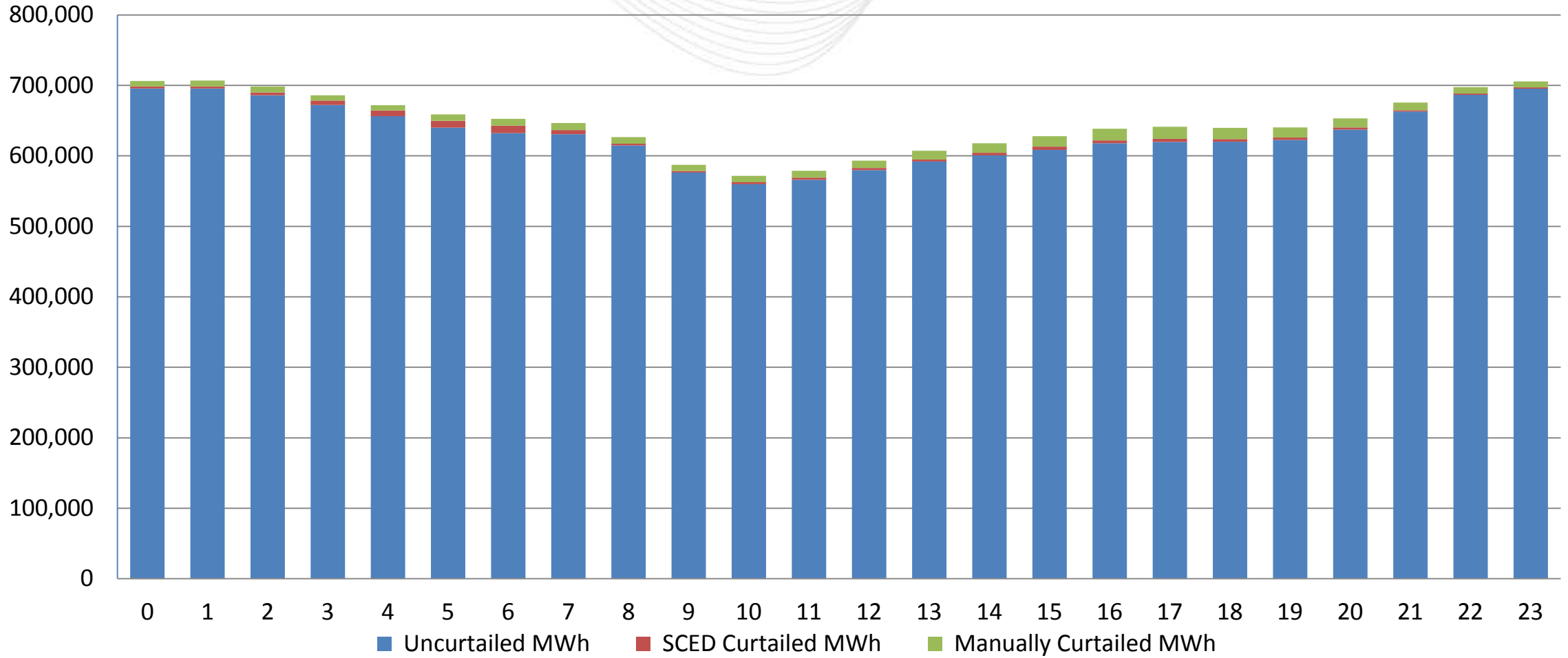
Hourly Wind Power Generation and Curtailments
