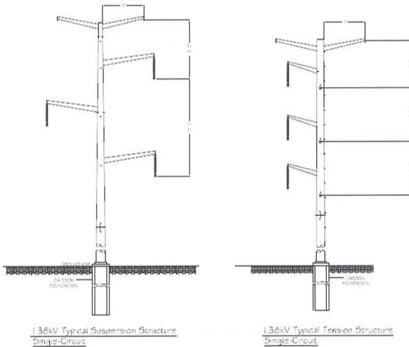
Figure C.1 - Typical 138kV Structure Types
