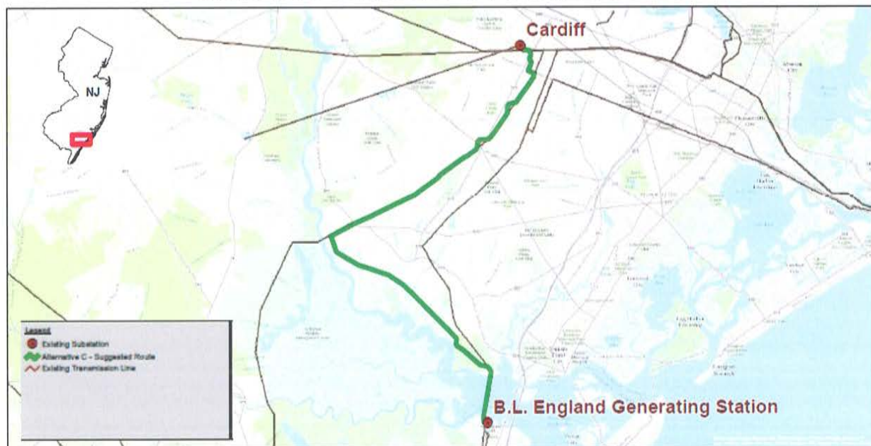
Figure C.1-1 - Proposed 138kV Transmission Line
