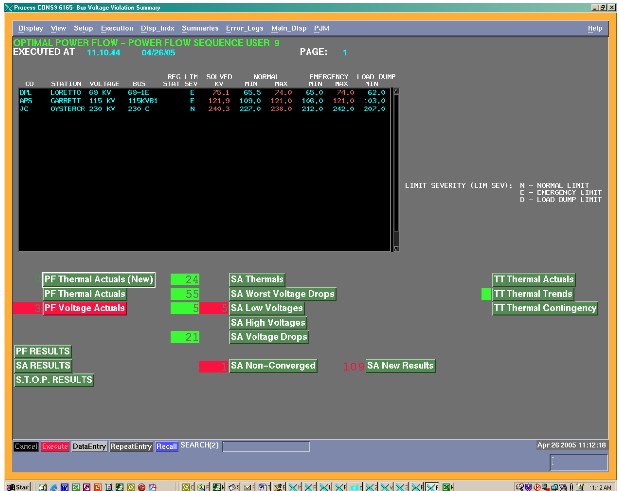
Exhibit 22: Voltage Actuals after Mitigation Steps
