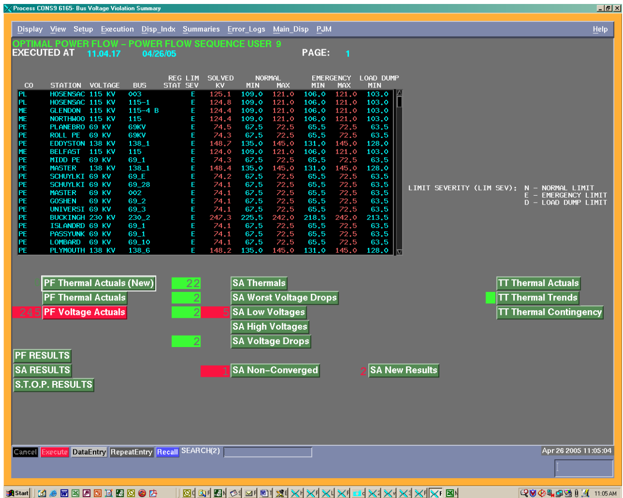
Exhibit 21: Voltage Actuals Prior to Mitigation Steps
