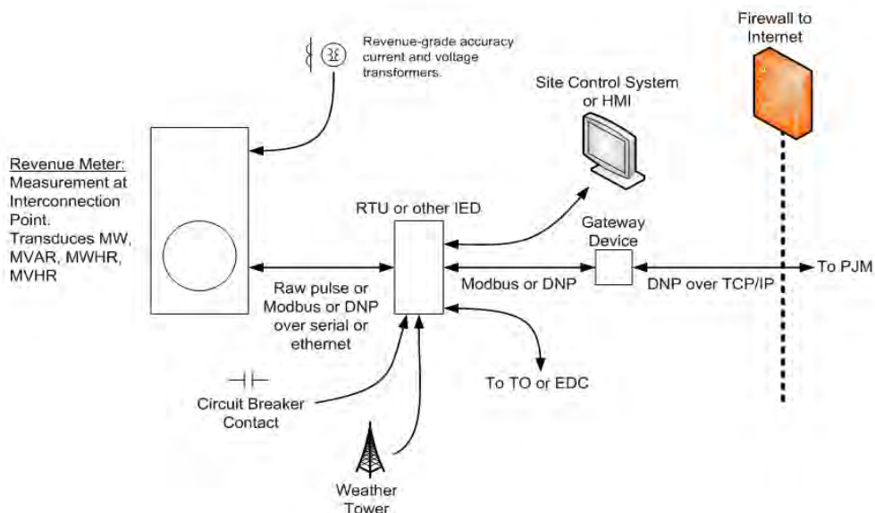
Exhibit 5: Typical Multi-Unit Metering and Data Flow Configuration
