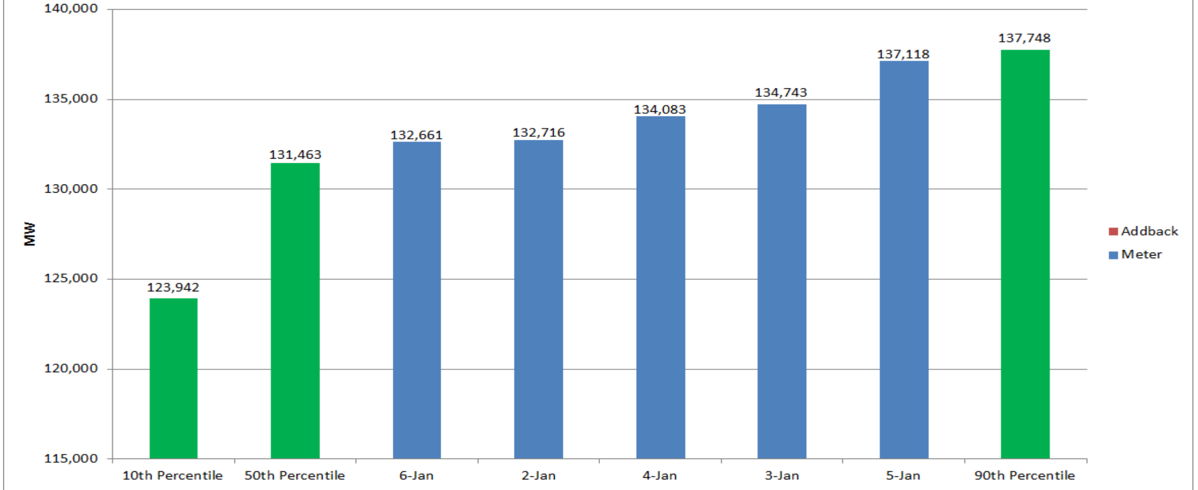
Comparison of PJM RTO Preliminary Winter Peaks to Forecasted Peak Levels - 2017/18
